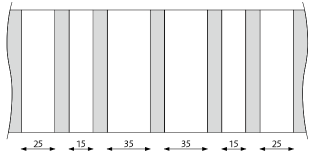
Pattern image
